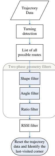
Fig. 3. The flow chart of our map-matching algorithm
