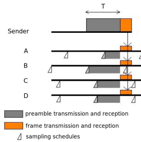
Fig. 3: WiseMAC broadcasting
